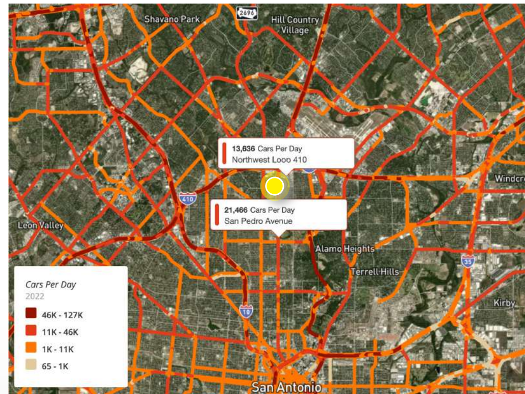
TRAFFIC COUNTS
