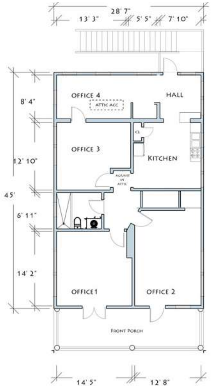
SECOND FLOOR
